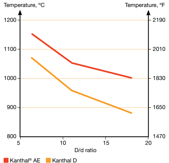
Permissible D/d (coil diameter/wire diameter) ratios as a function of wire temperature in supported coil elements
